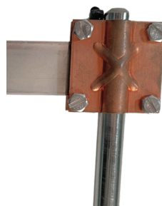
Ref. 16125 Copper connecting collar For flat conductors
